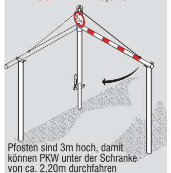
LKW-SCHRANKE 3,5–6 m
